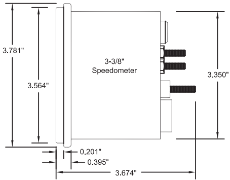
3 3/8" Speedometer
