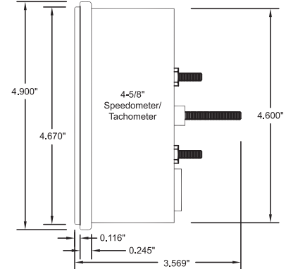
4 5/8" Speedometer / Tachometer
