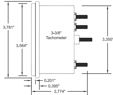
3 3/8" Tachometer
