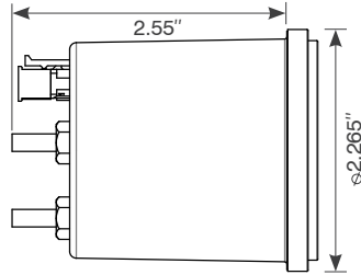
2 1/8" Full-sweep Gauges
