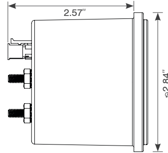
All 2 5/8" Gauges
