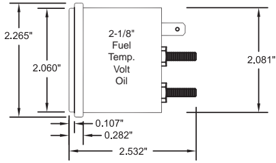
2 1/8" Short-sweep Gauges
