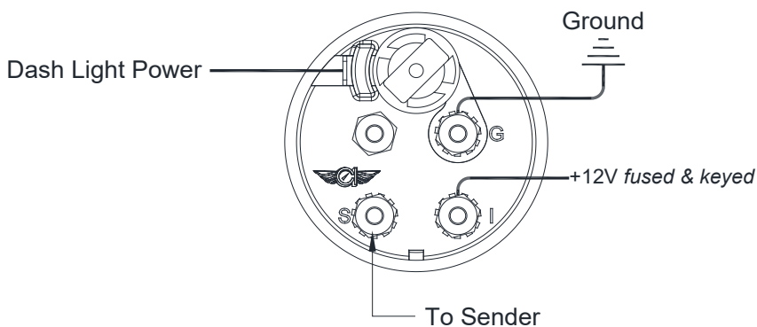
Back of Gauge
