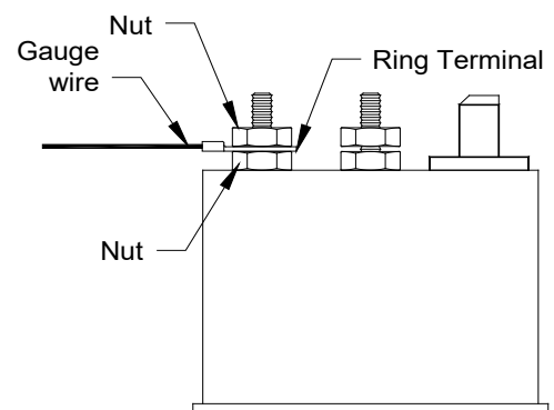
Side of Gauge
