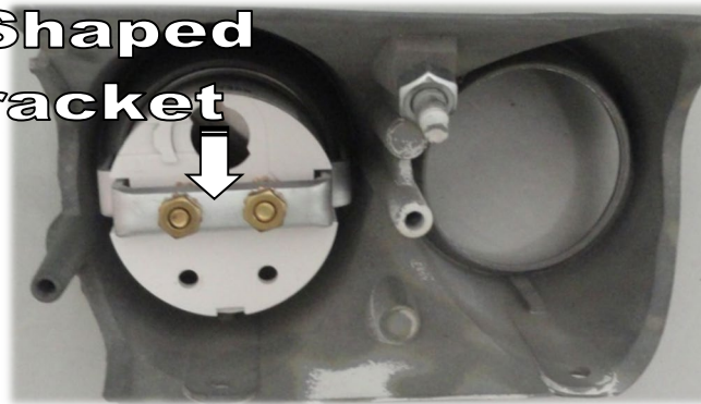
Partially Assembled Side Gauge Pod
